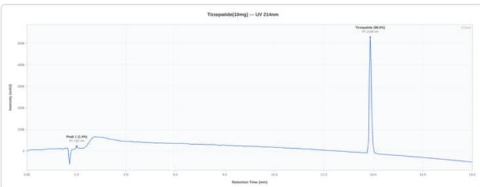
HPLC Chromatogram
