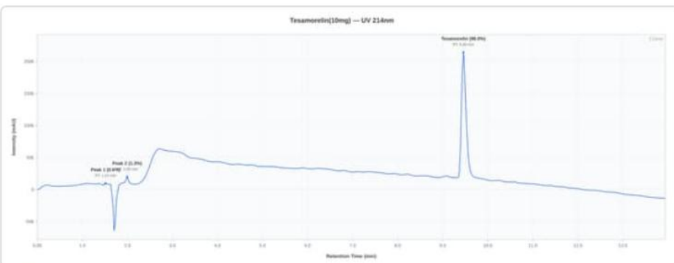
HPLC Chromatogram
